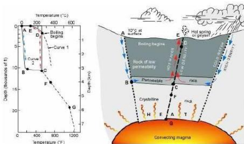
Gambar 4. https://geochemist.wordpress.com/2008/10/09/sistem-reservoir-panasbumi/
