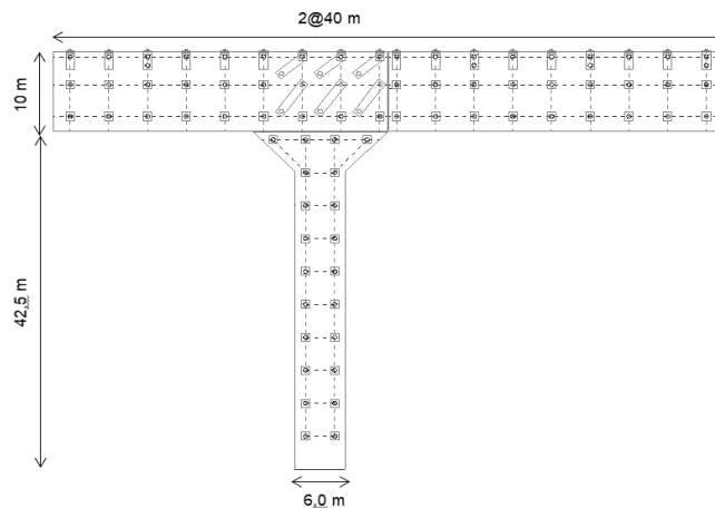
Gambar 3. Layout Dermaga Lampia
